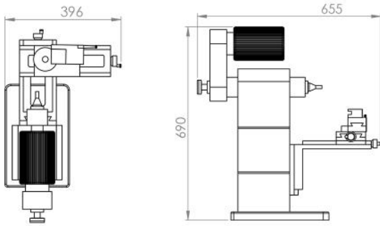
Outside Lathe Machine
